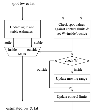
Figure 3: Flip-Flop Filter
